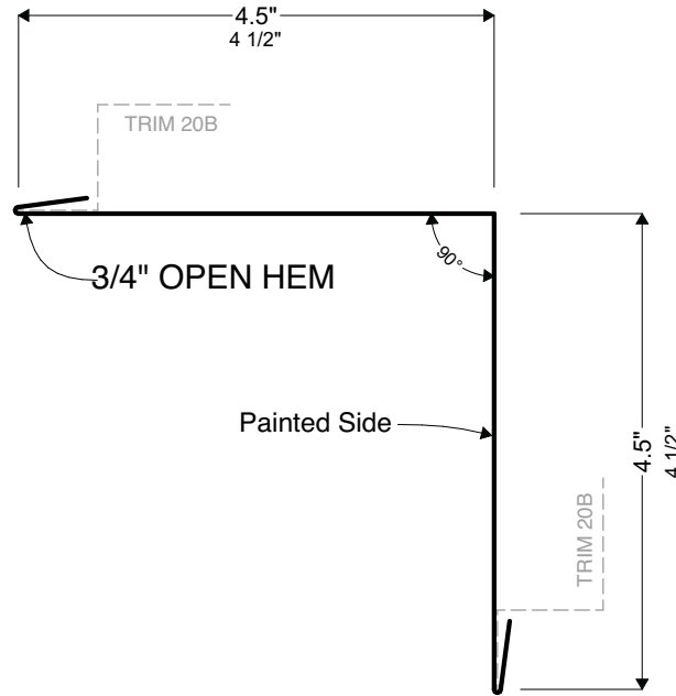
A1 Profile Section Detail Scale: 6" = 1'-0"
