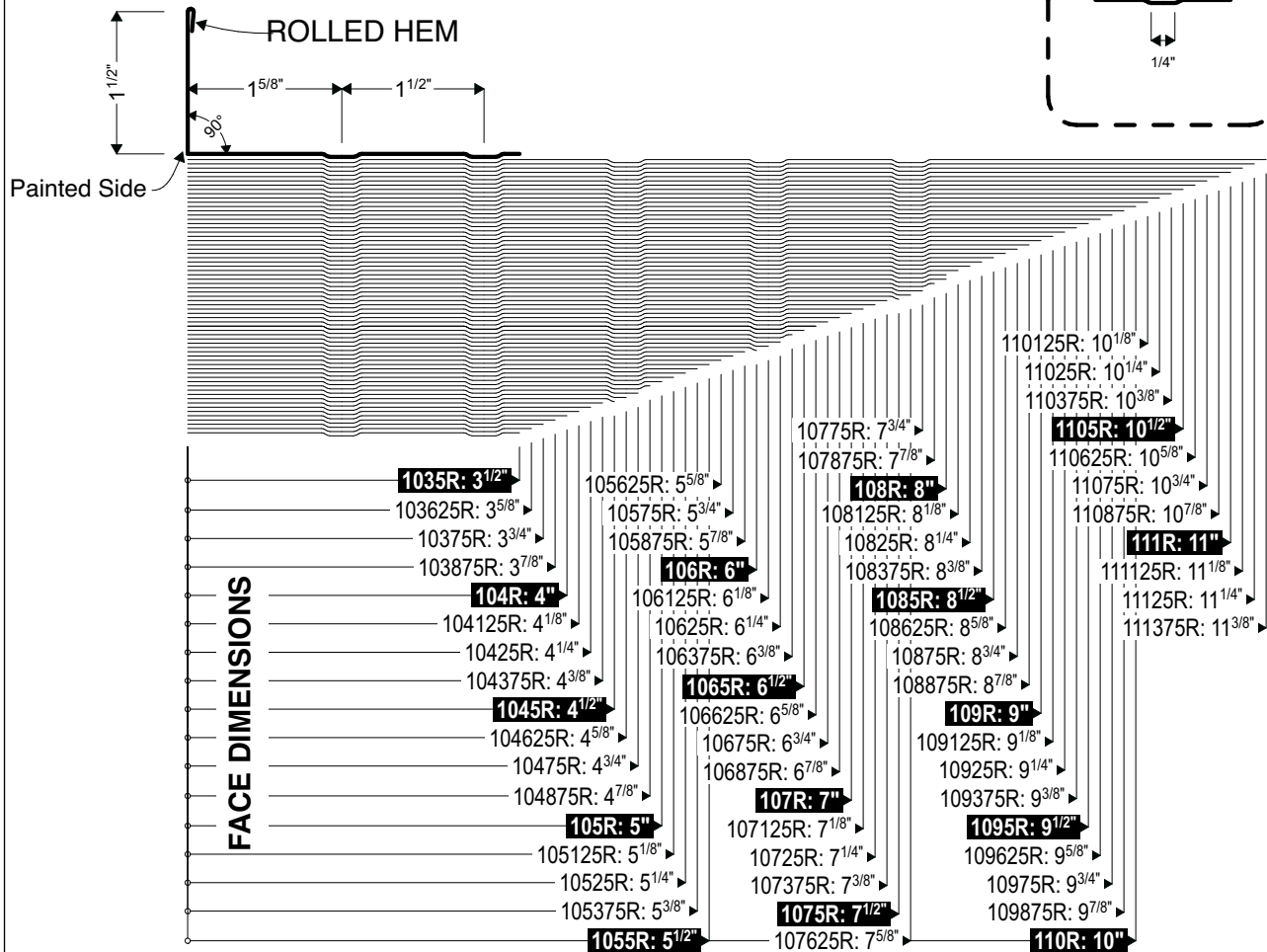
A1 Profile Section Detail Scale: 6" = 1'-0"
