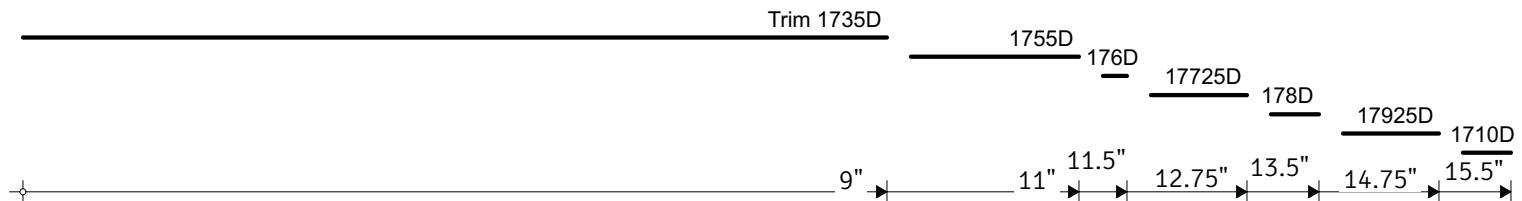
B1 Profile Flat Width Required Scale: 6" = 1'-0"
