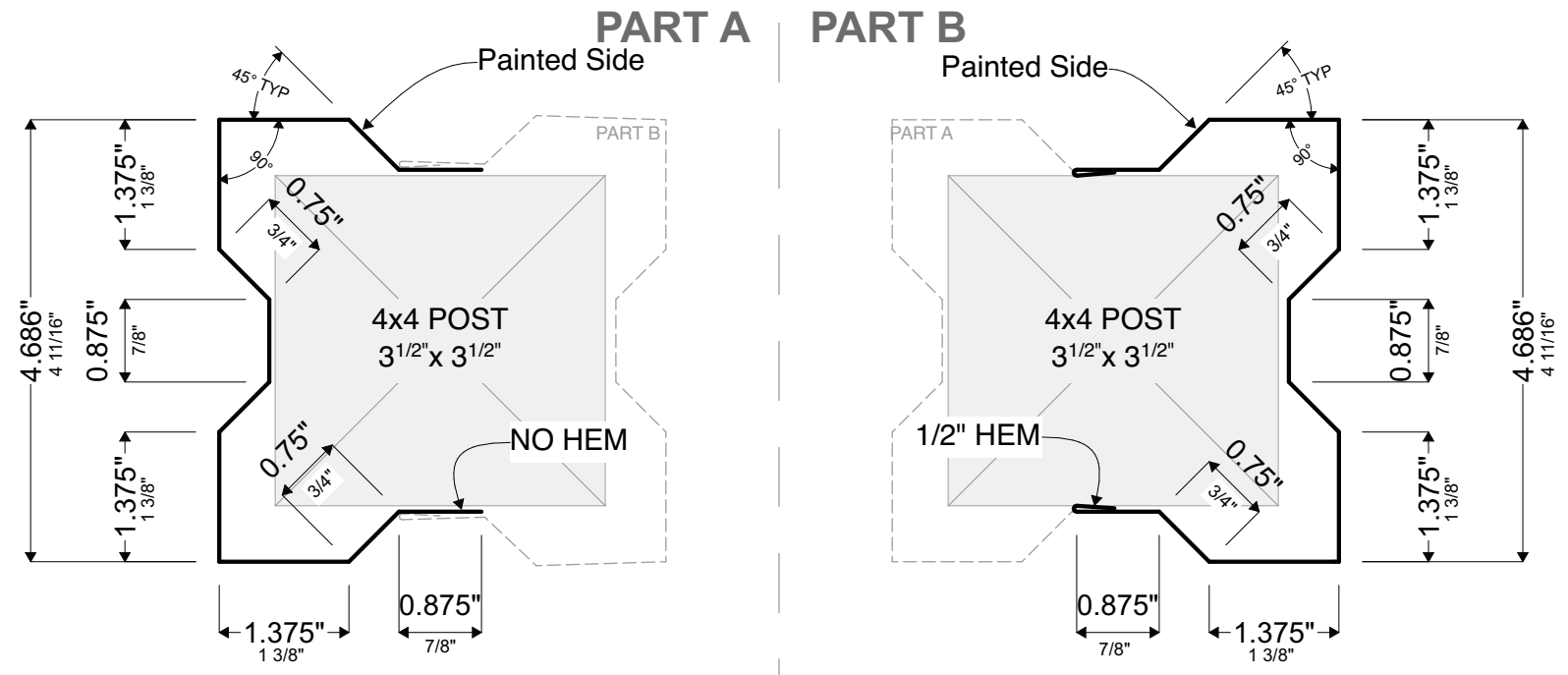
A1 Profile Section Detail Scale: 6" = 1'-0"
