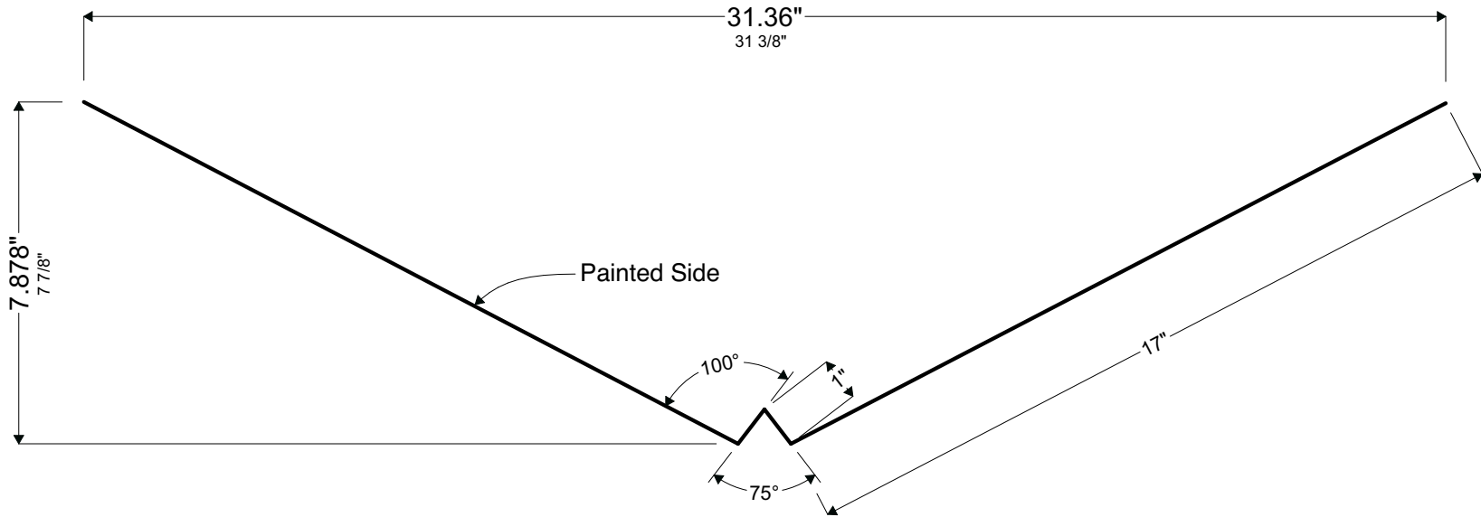
A1 Profile Section Detail Scale: 3" = 1'-0"
