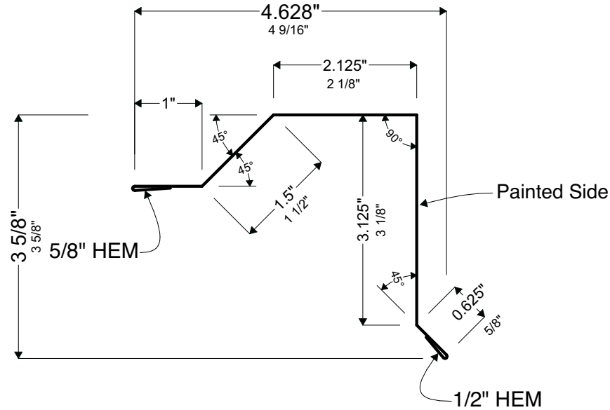
A1 Profile Section Detail Scale: 6" = 1'-0"
