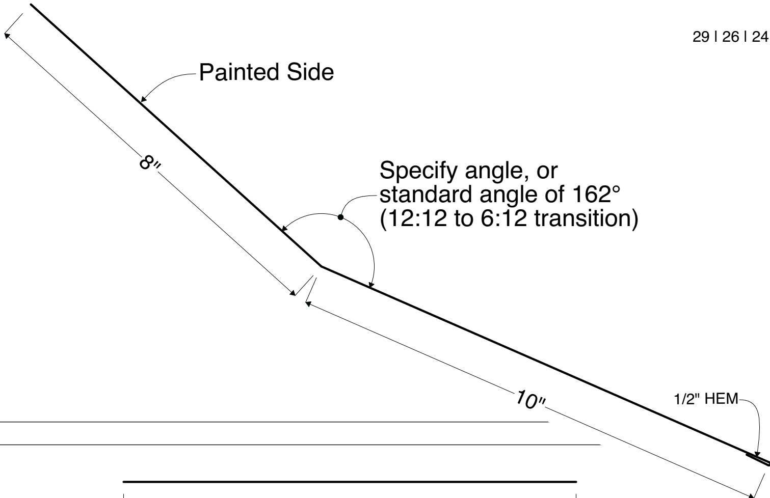
A1 Profile Section Detail Scale: 6" = 1'-0"
